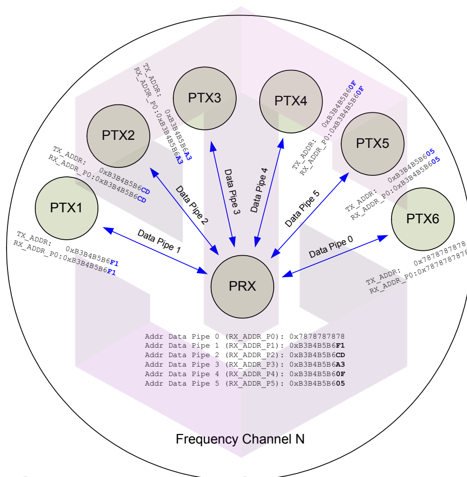
Figure 12. Example of data pipe addressing in MultiCeiver™
