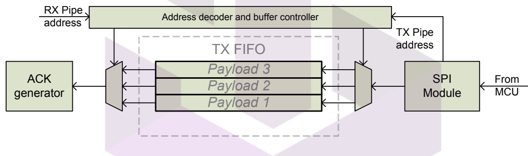
Figure 7. TX FIFO (PRX) with pending payloads
